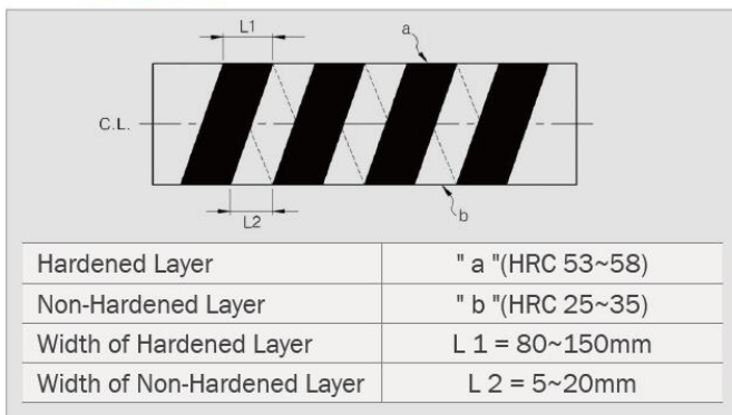
“ A ” Detail : Spiral Characteristy (Imagine “Spring”)
