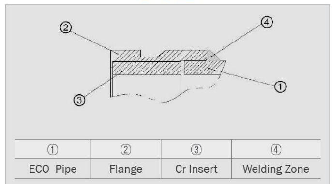
“ B ” Detail
