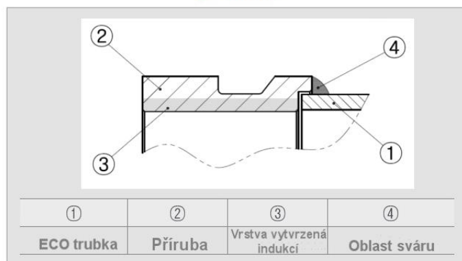
“ B ” Detail
